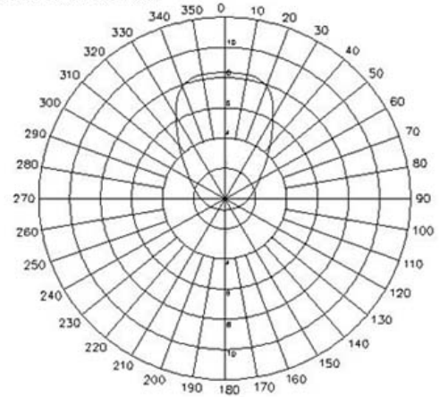
E-PLANE FIELD PATTERNS
