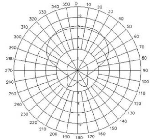
E-PLANE FIELD PATTERNS
